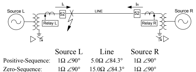
Fig. 12. System single-line diagram for sensitivity study.
