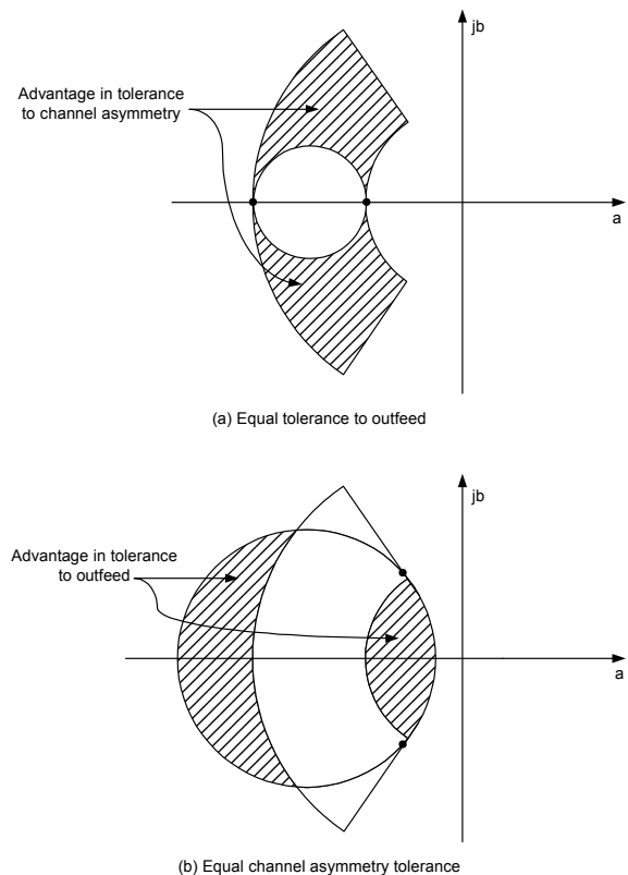
Fig. 9. Advantages of the new characteristic over the percentage differential characteristic
