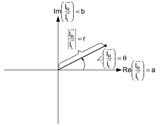
Fig. 1. \alpha -Plane represents the complex ratio of \bar{I}_R / \bar{I}_L
