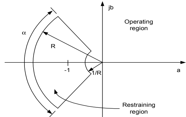
Fig. 8. Characteristic of the new differential element in the current-ratio plane
